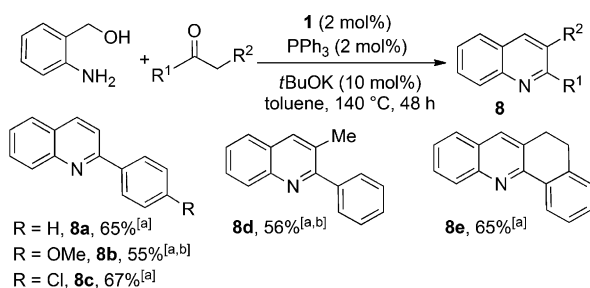
Scheme 2. Iron-catalyzed modified Friedländer annulation reaction. [a] Yields of isolated products. [b] 30 mol% of t BuOK was used.
