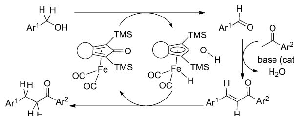
Scheme 1. Iron-catalyzed \alpha -alkylation of ketones with alcohols.
